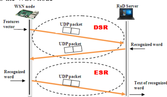
Fig. 9 CTP Workflow
