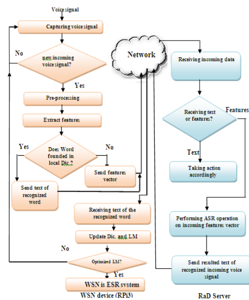
Fig. 10 Suggested Algorithm Flowchart.
